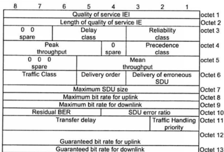
Figure 10.5.138/3GPP TS 24.008: Quality of service information element
